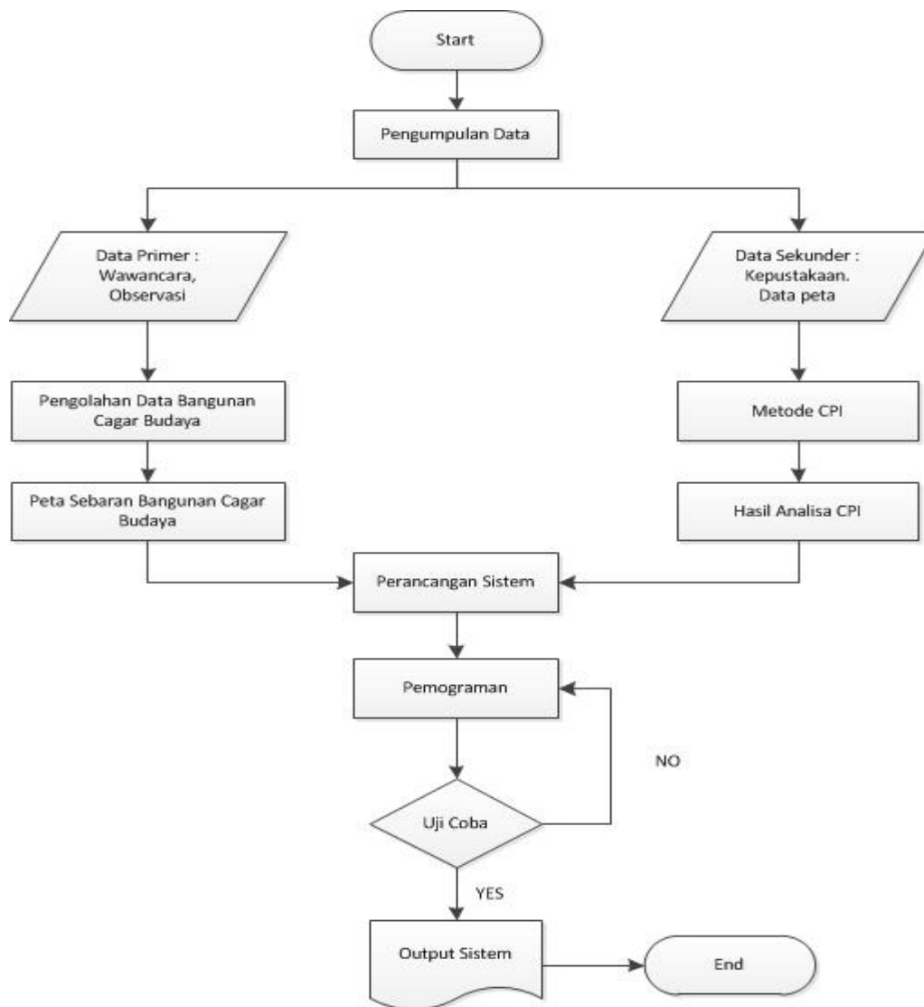
Gambar 1 Metode Penelitian
